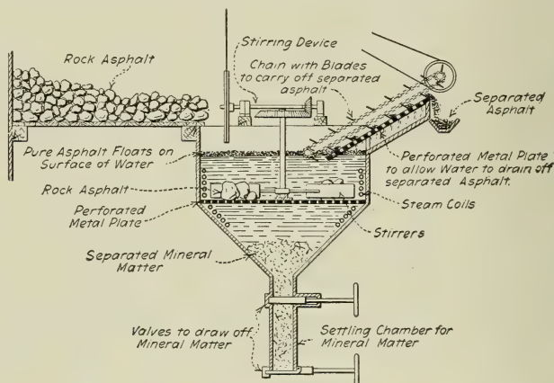
FIG. 26.—Apparatus for Separating Soft Asphalt from Sand by Means of Water.
